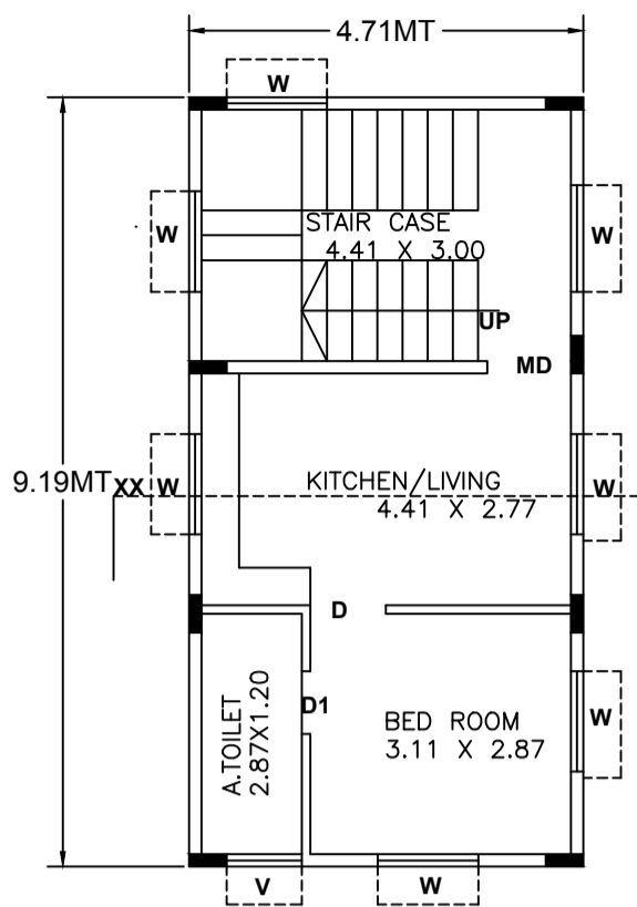
PROPOSED TYPICAL FIRST & SECOND FLOOR PLAN
